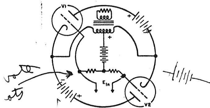
Fig. 5 — Simplified Diagram Circlotron Circuit
