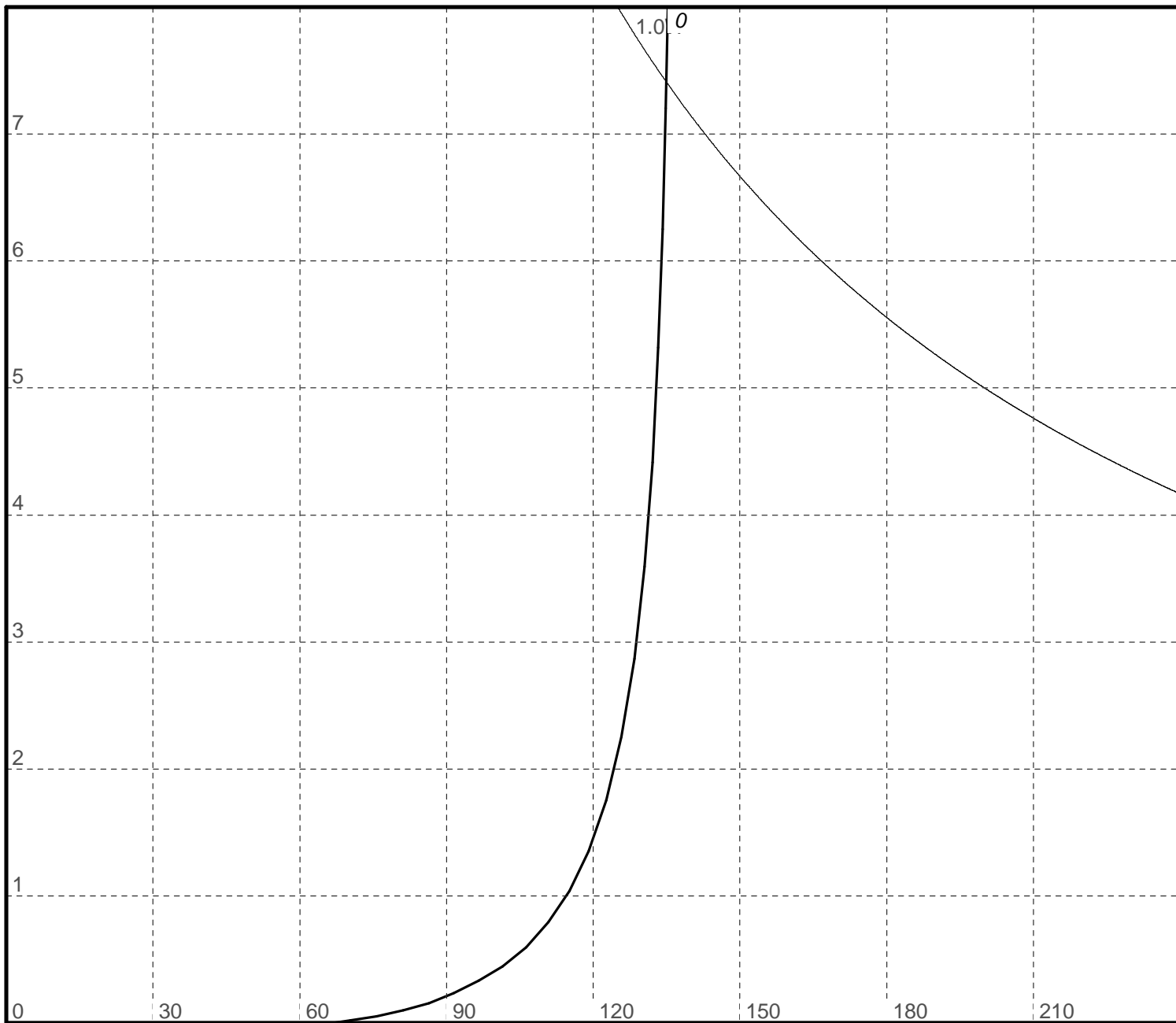
S20K75 VDR. Shown single ended, but bidirectional.
