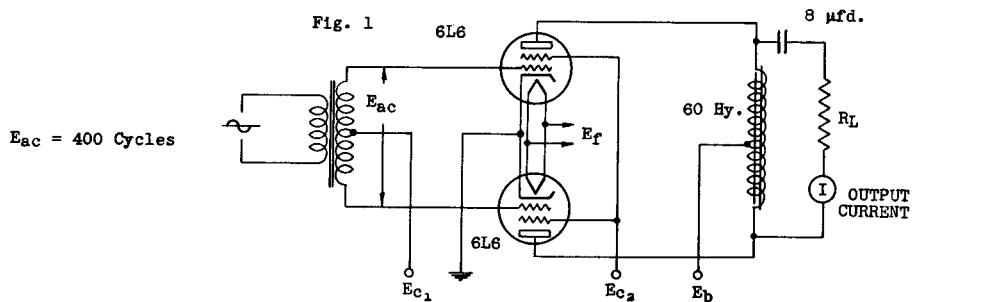
CIRCUIT FOR CLASS AB OPERATION WITH POWER DRIVERS
